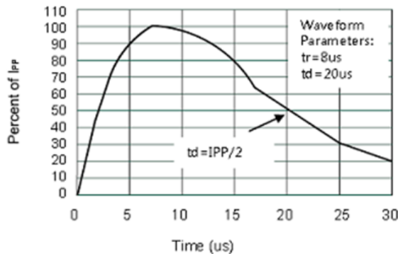
FIGURE 1 Pulse Waveform
